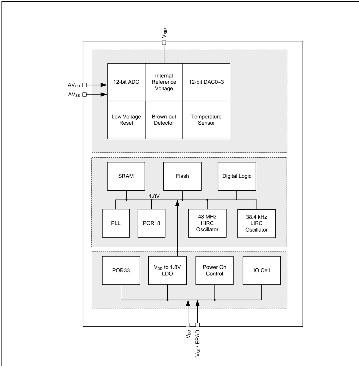
Figure 6.2-6 NuMicro® M029G/M030G/M031G Power Distribution Diagram
