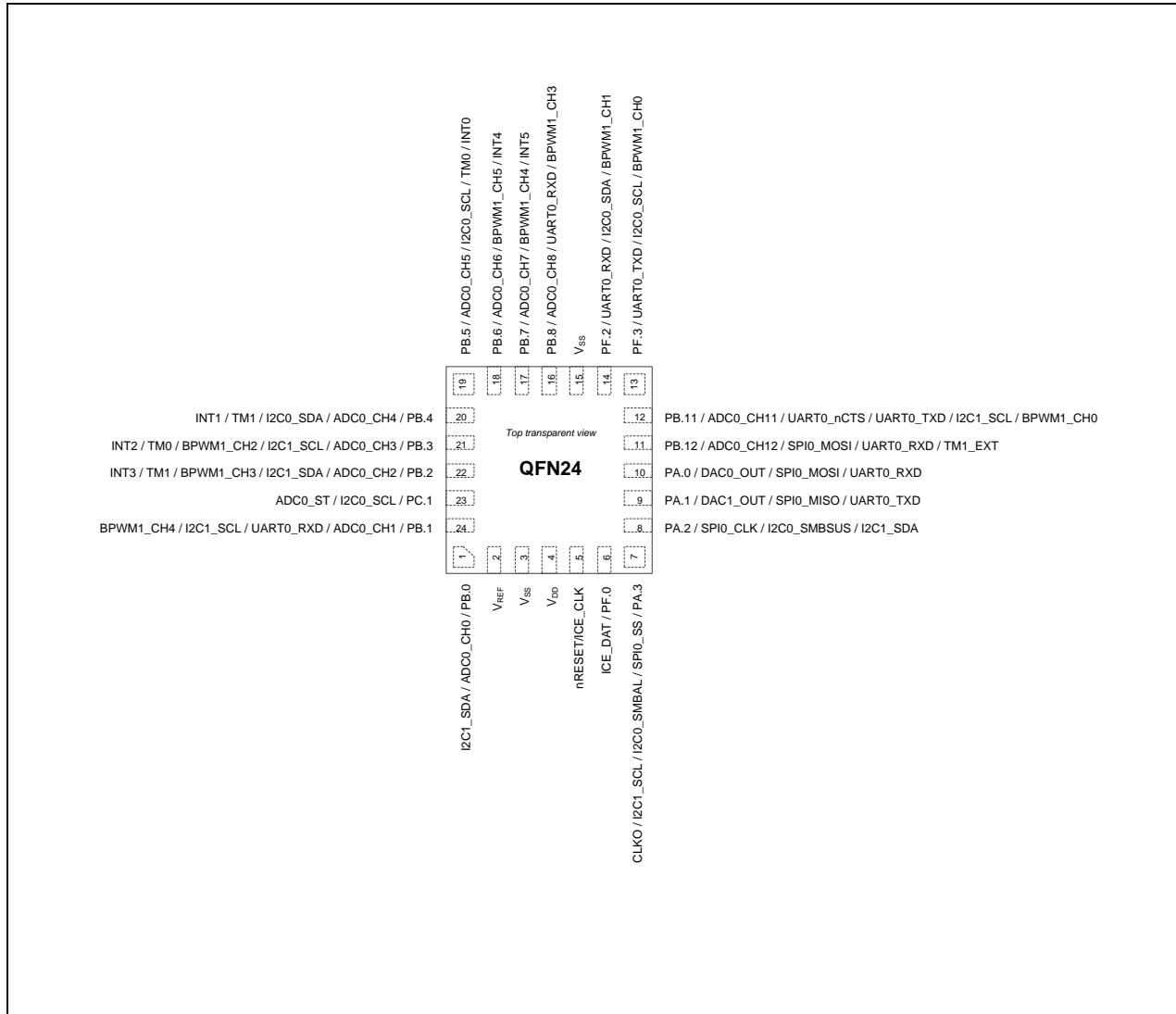
Figure 4.1-3 M029G Series QFN 24-pin Multi-function Pin Diagram
